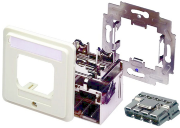
AMP CO Ultra Outlet Installation Kit, DIN 68 x 68, pure white
