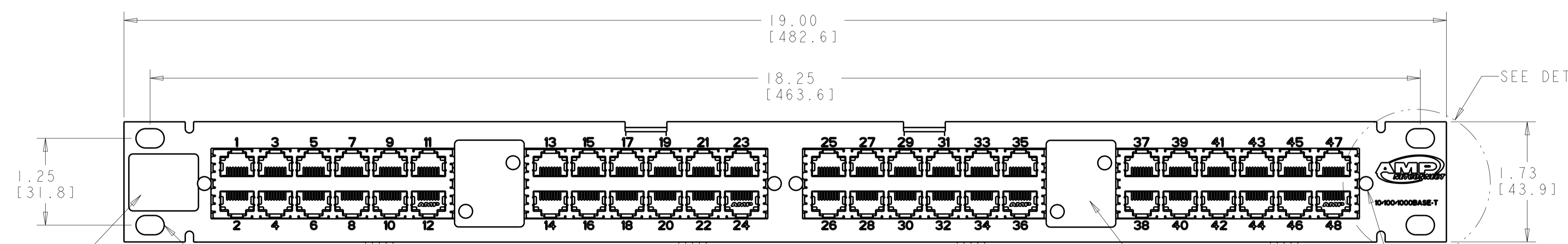
FRONT VIEW
