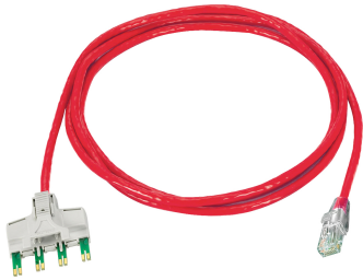
Ultim8 Copper Patch Cord, 4-pair to RJ45, category 6, red, 25 ft
