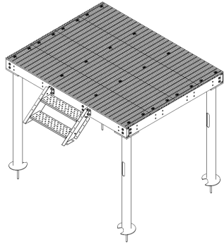
Equipment Platform, 8 ft x 10 ft, base with four 15ft x 6in OD Helicals
