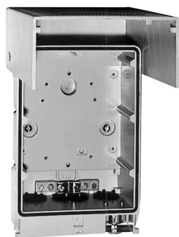
LSA-PLUS® KRONECTION box A-30, unloaded, 30-pairs
