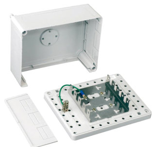
LSA-PLUS® Junction Box, Low profile, with earthing, 250/5, 50-pairs
