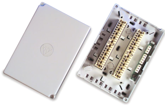
LSA-PLUS® Connection Box, Low profile, 201D, 20 pairs
